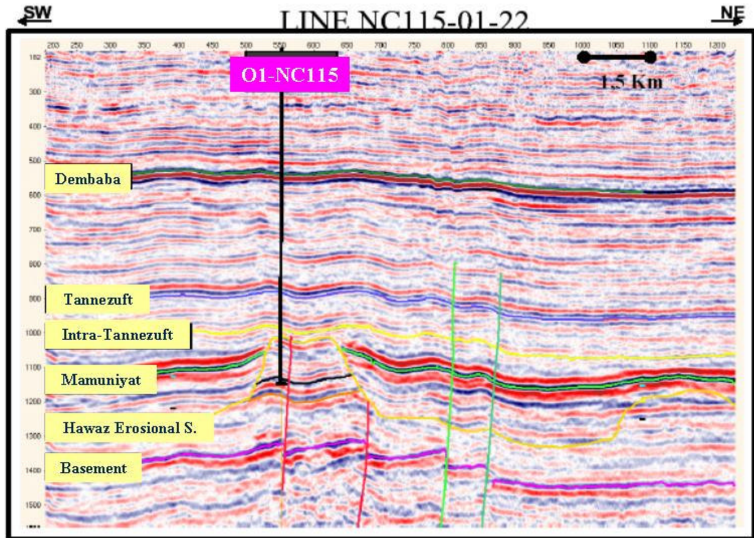
SEISMIC LINE WITH THE WELL LOCATION
