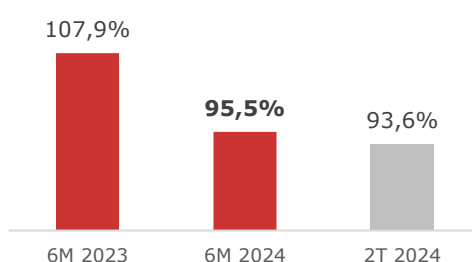
COMBINED RATIO
